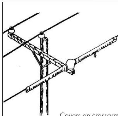
Covers on crossarm construction
