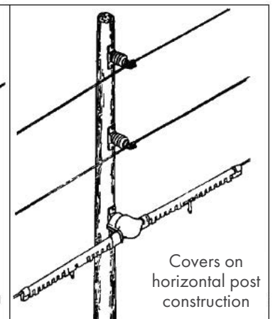
P406-0184 without Grip-All Adapter for rubber glove application
